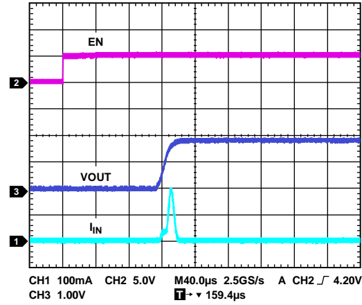
Figure 30. LDO Startup, V_{OUT3} = 1.8 V
