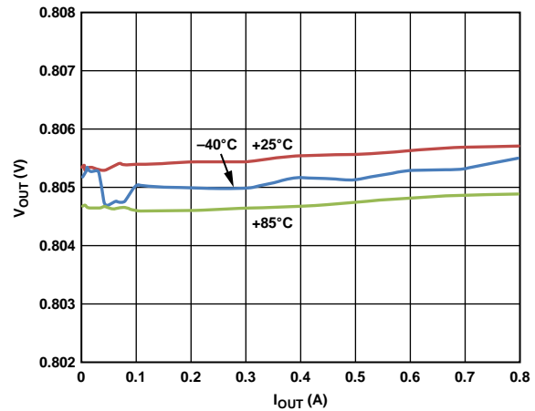
Figure 8. BUCK1 Load Regulation Across Input Voltage, V_{IN} = 3.6\text{ V} , V_{OUT1} = 0.8\text{ V} , PWM Mode
