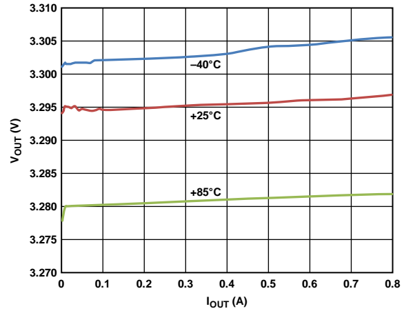
Figure 6. BUCK1 Load Regulation Across Temperature, V_{IN} = 4.2\text{ V} , V_{OUT1} = 3.3\text{ V} , Auto Mode
