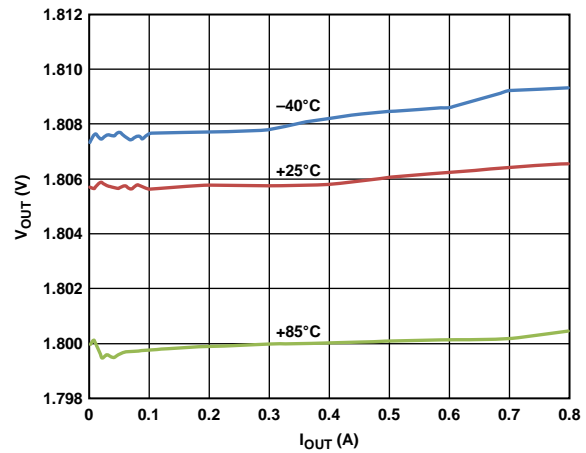
Figure 7. BUCK2 Load Regulation Across Temperature, V_{IN} = 3.6\text{ V} , V_{OUT2} = 1.8\text{ V} , Auto Mode
