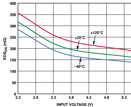
Figure 32. NMOS R_{DS(on)} vs. Input Voltage Across Temperature
