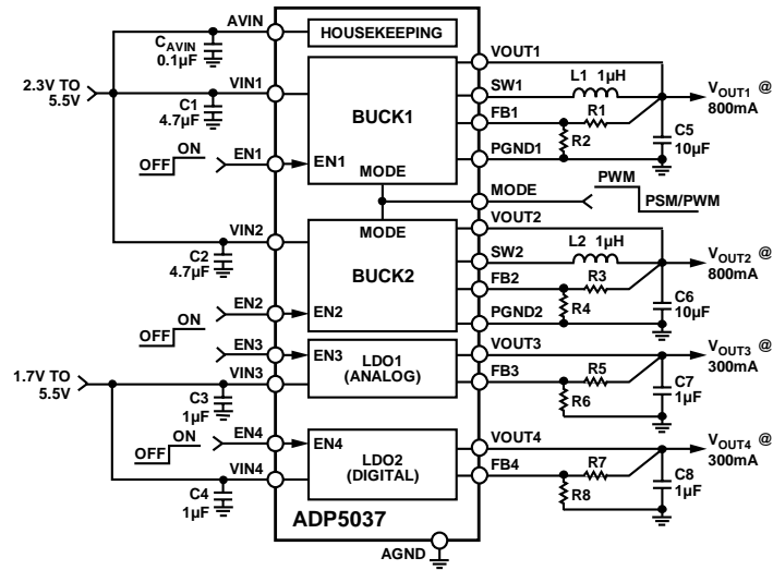
Figure 53. ADP5037 Adjustable Output Voltages with Enable Pins
